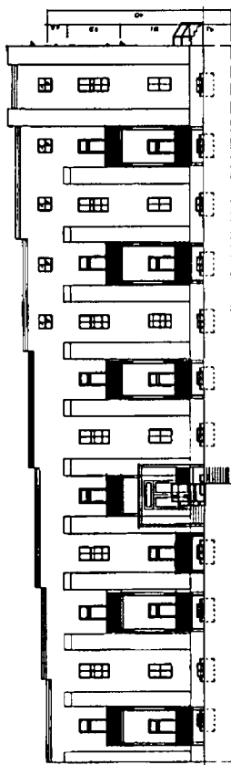
WEST ELEVATION
