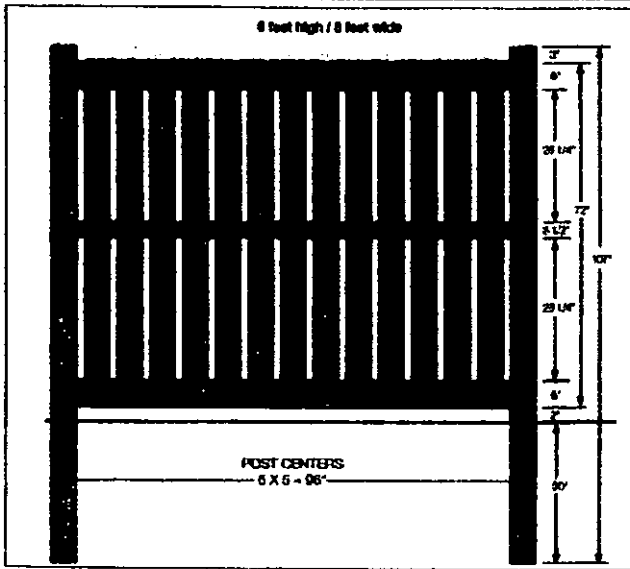
FENCE DETAIL
