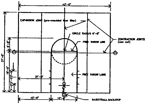
HALF BASKETBALL COURT PLAN
