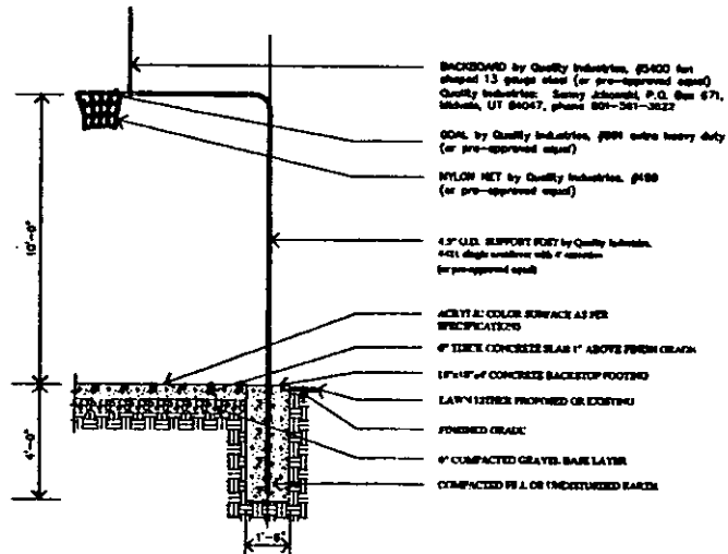
BASKETBALL BACKSTOP DETAIL
