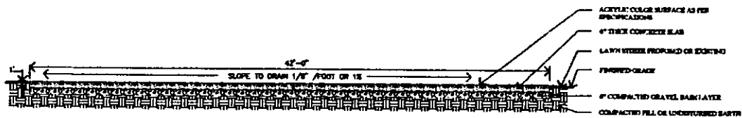
BASKETBALL COURT CROSS SECTION
