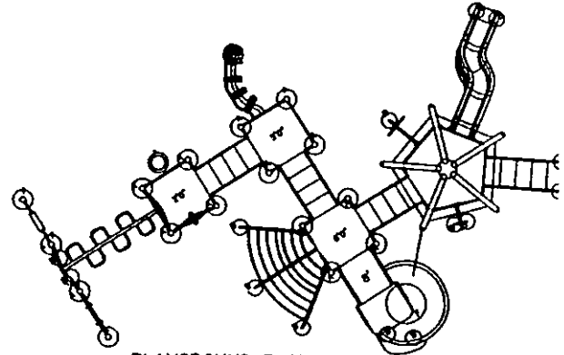
PLAYGROUND PLAN VIEW
