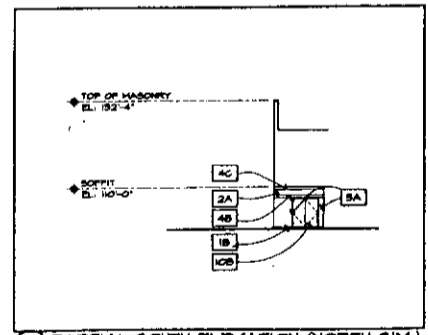
5 PARTIAL SOUTH ELEVATION (NORTH SIM) AS 1/16" = 1'-0"
