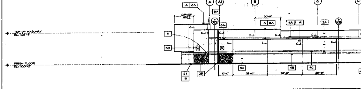
3 SOUTH ELEVATION (LEFT) AS 1/16" = 1'-0"
