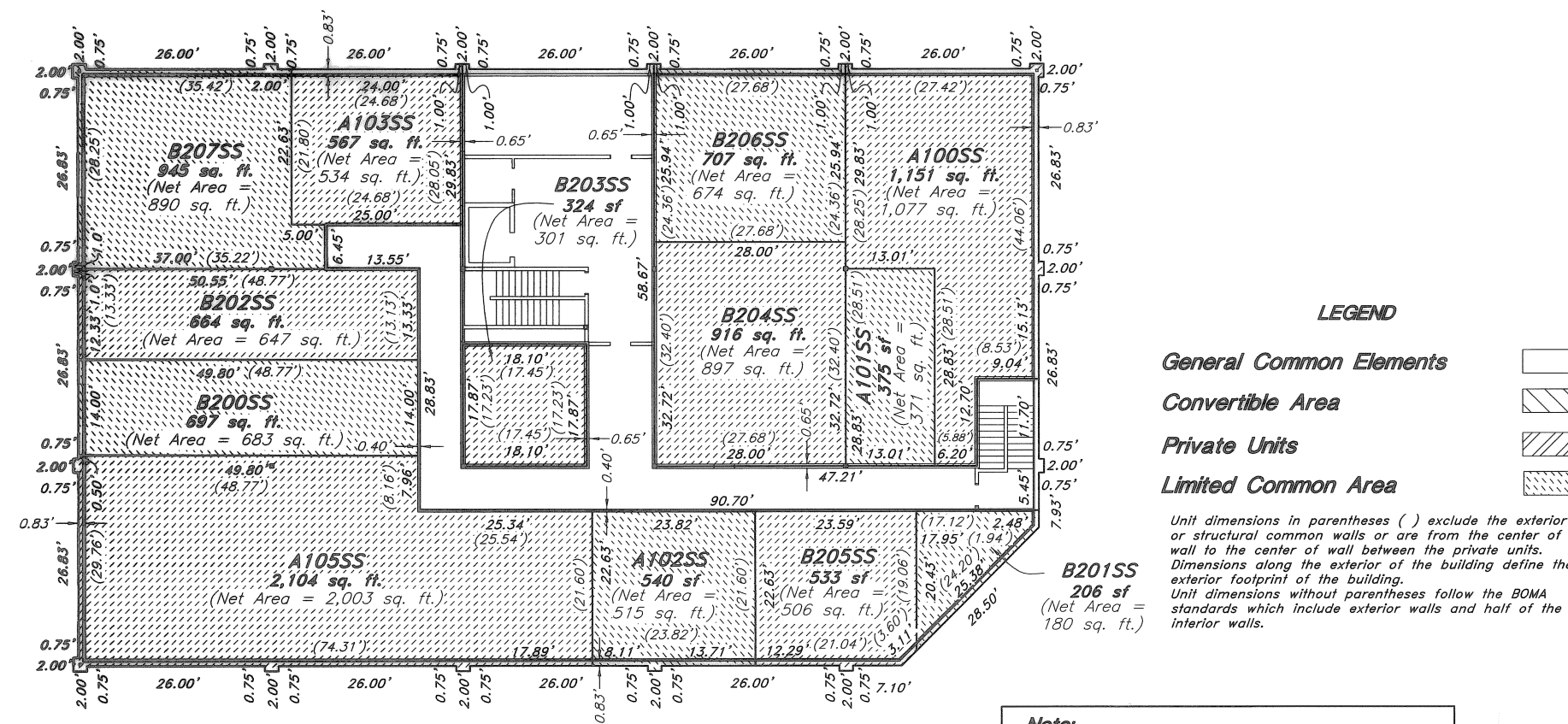
Basement Level Foot Print 12,046 sq. ft. Scale: 1" = 16'
