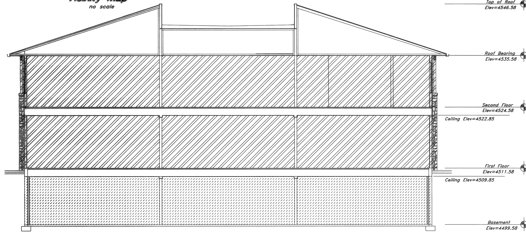
Vertical Section Scale: 1" = 10'
