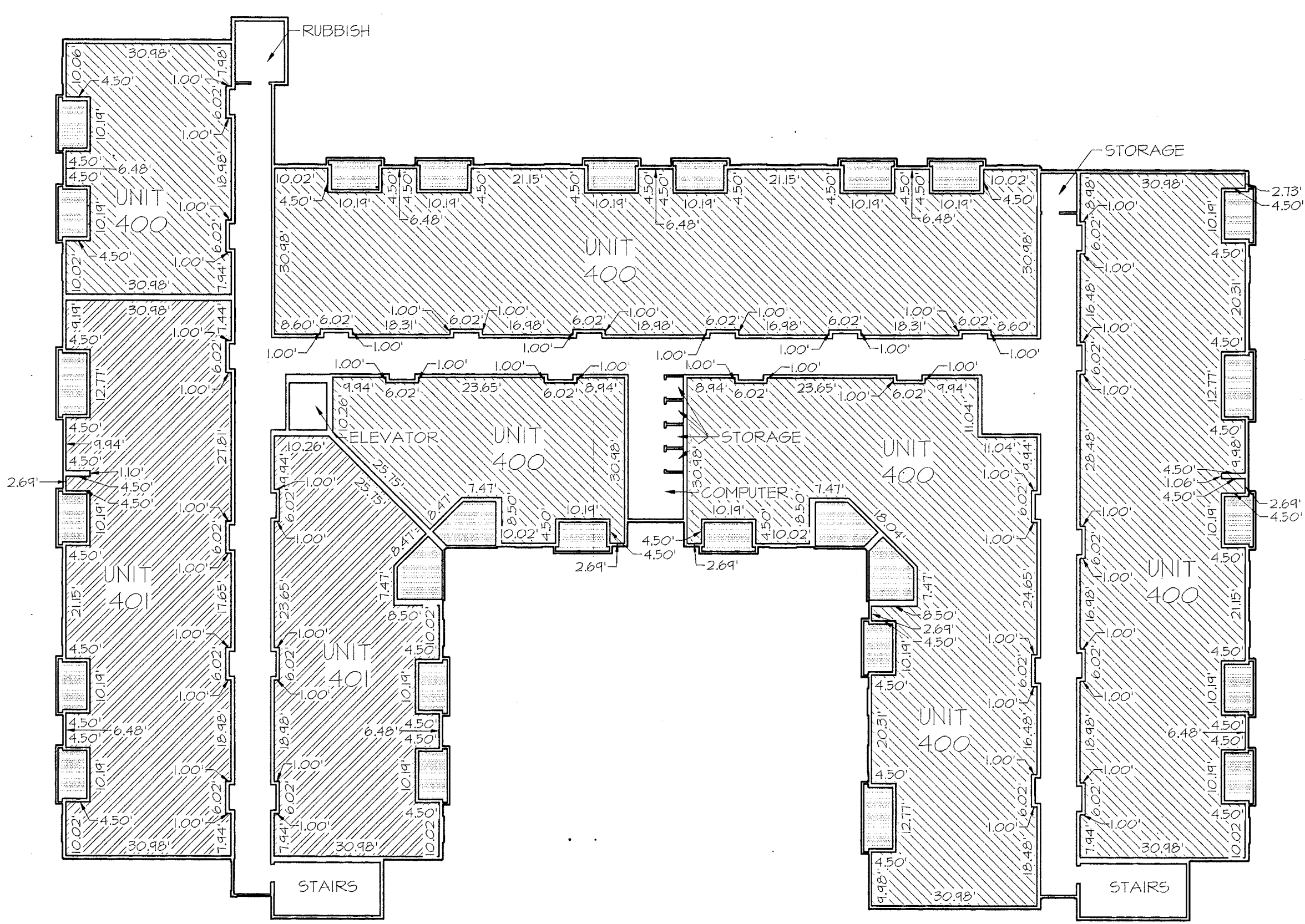
FOURTH FLOOR PLAN SCALE: 1" = 20'
