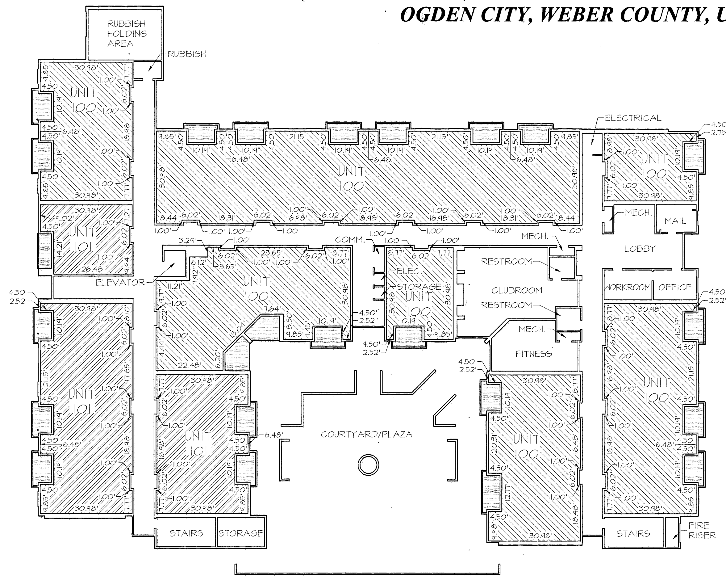
FIRST FLOOR PLAN SCALE: 1" = 20'
