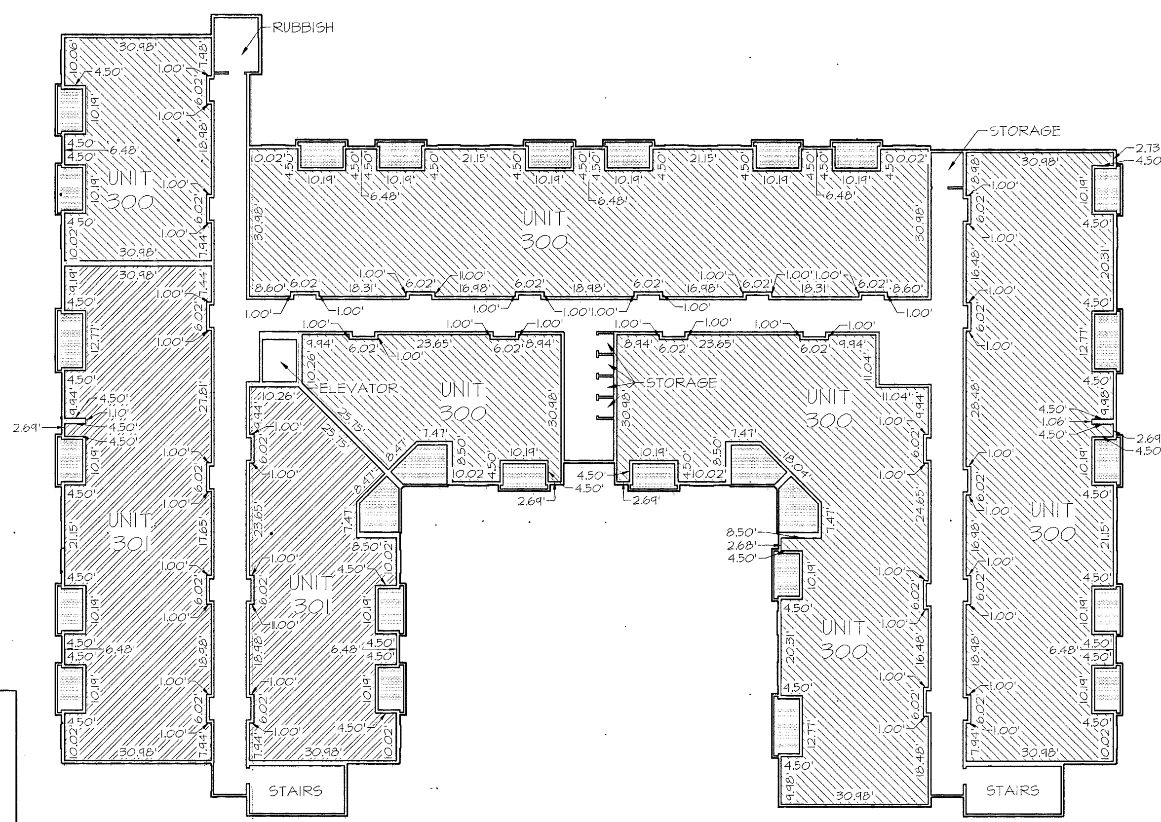
THIRD FLOOR PLAN SCALE: 1" = 20'
