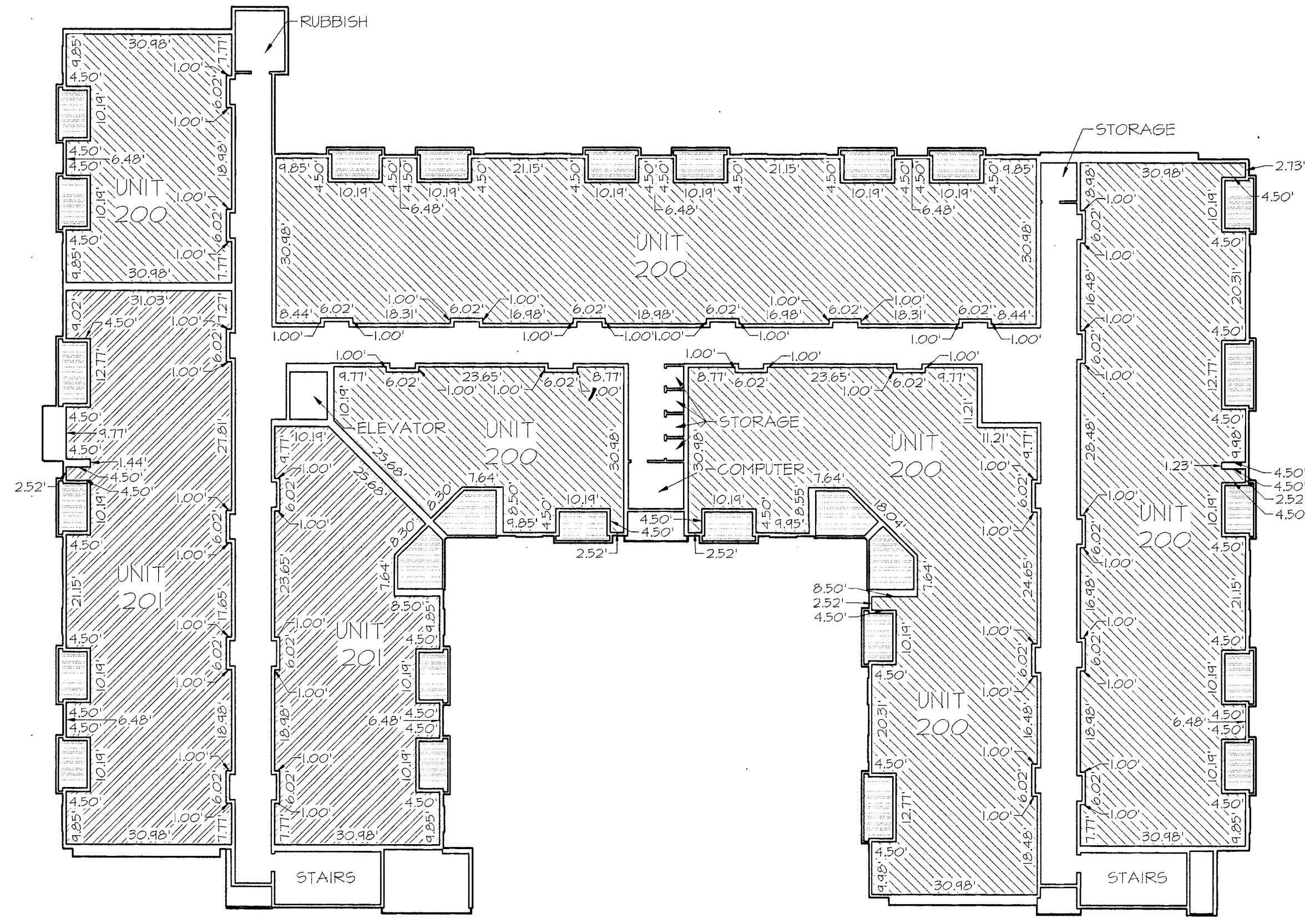
SECOND FLOOR PLAN SCALE: 1" = 20'
