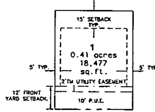
TYPICAL LOT SETBACKS DETAIL (N.T.S.)
