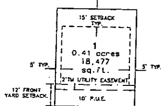
TYPICAL LOT SETBACKS DETAIL (N.T.S.)
