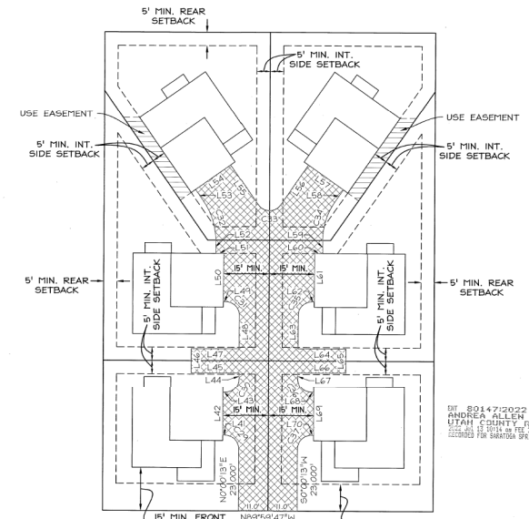
COTTAGE LOTS 1-6 SETBACK AND EASEMENT DETAIL SCALE: 1"=20'
