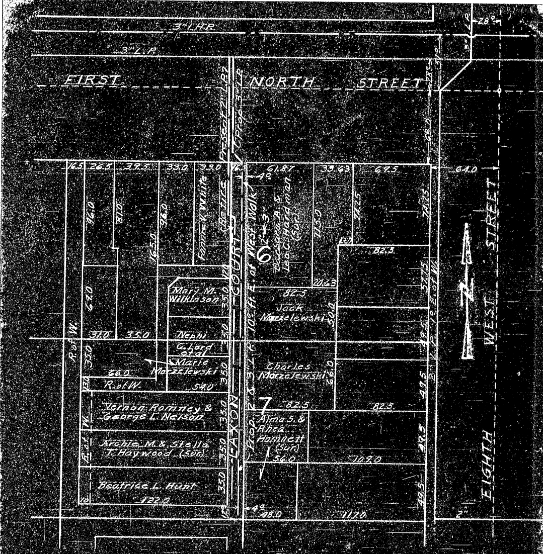
MOUNTAIN FUEL SUPPLY COMPANY MAP SHOWING PARTS OF LOTS 6 & 7, BLOCK 64, PLAT C, S. L. C. SURVEY APRIL 17, 1953 F. A. K. SCALE: 1" = 60'
