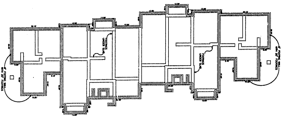
FOUNDATION PLAN (BUILDING 5)
