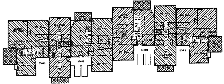
FIRST FLOOR PLAN (BUILDING 5)
