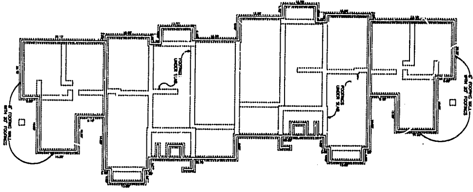
FOUNDATION PLAN (BUILDING 7)
