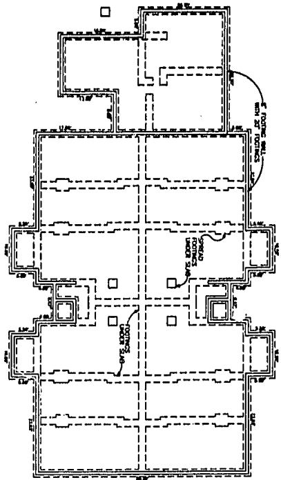
FOUNDATION PLAN (BUILDING 4)
