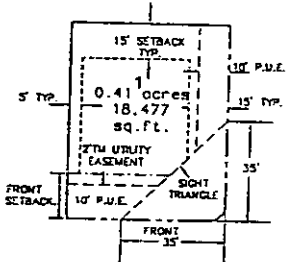
TYPICAL CORNER LOT SETBACKS DETAIL (N.T.S.)
