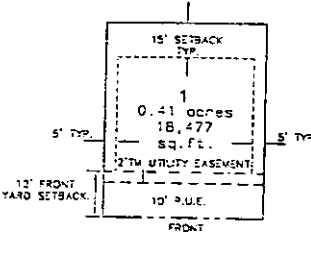
TYPICAL LOT SETBACKS DETAIL (N.T.S.)
